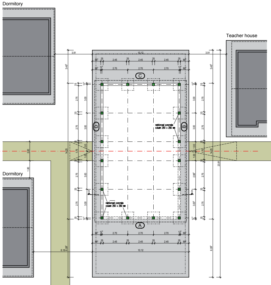
Ground-floor plan
